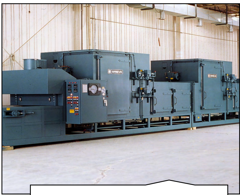
791 Custom Belt Conveyor Zones Exhaust Hood
