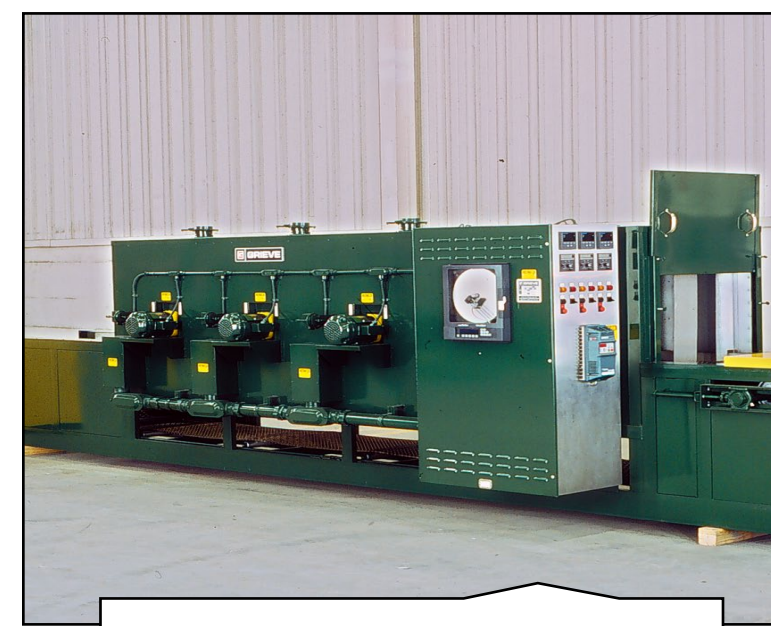
794 Custom Belt Conveyor Zones
