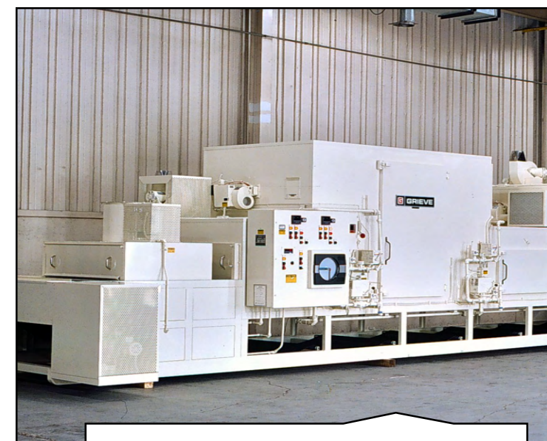
810 Custom Belt Conveyor Zones Cooling
