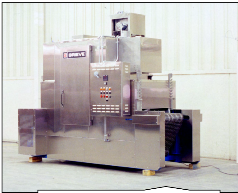
937 Custom Belt Conveyor Stainless Exterior
