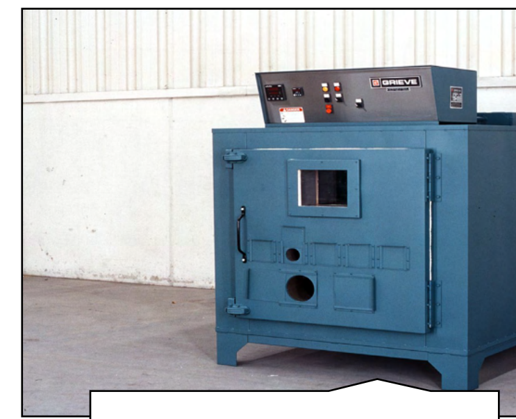
985 Custom Universal Ovens Door Modification
