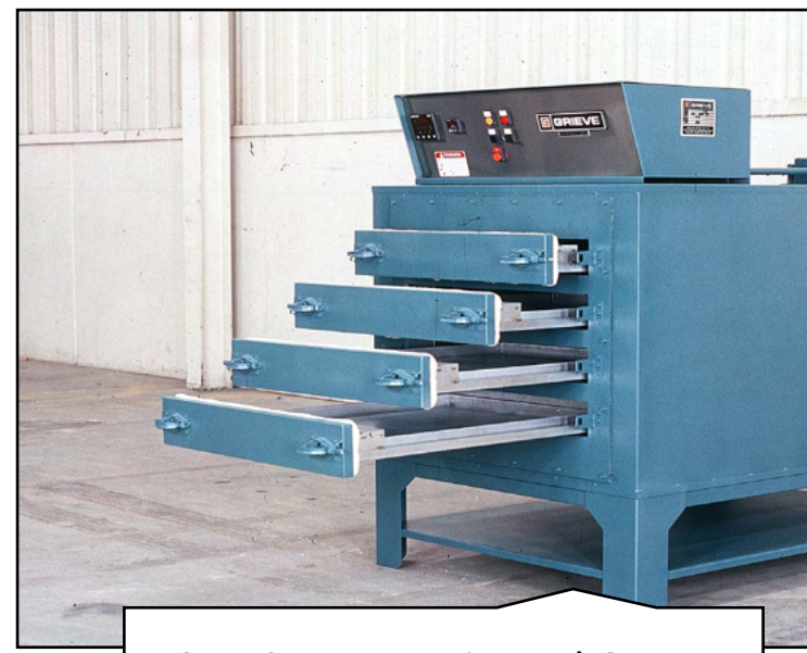
977 Custom Universal Ovens Drawers
