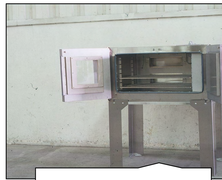
983 Custom Bench Oven Door Modification
