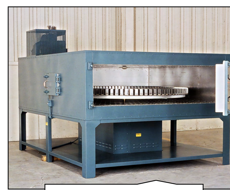
815 Custom Rotary Hearth Vertical Airflow
