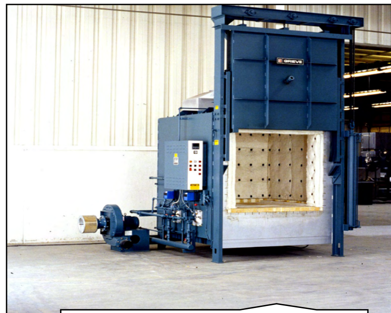
908 Custom Heavy Duty Furnaces Gas Fired Furnace
