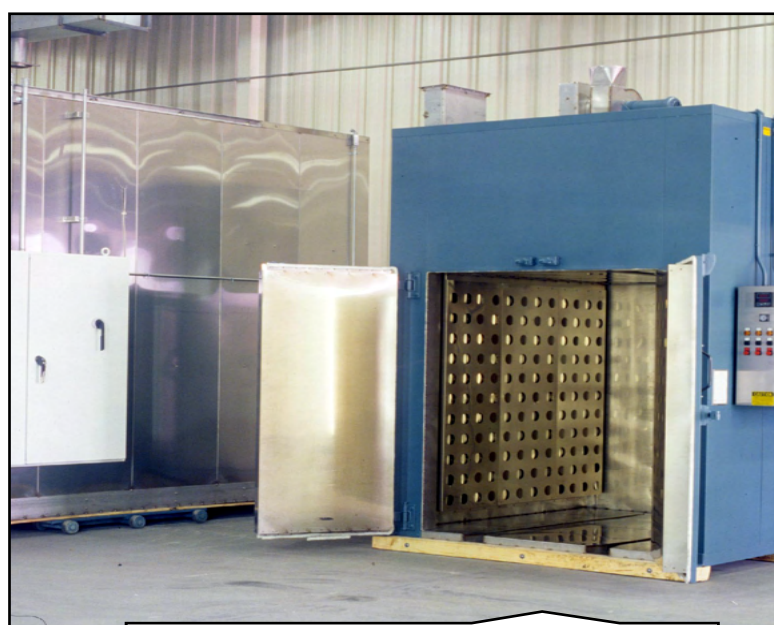
948 Custom Walk In Ovens Gas Fired Top Heat Chamber
