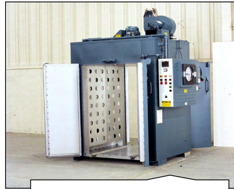
860 Custom Truck Ovens Top Heat Chamber Door Modification
