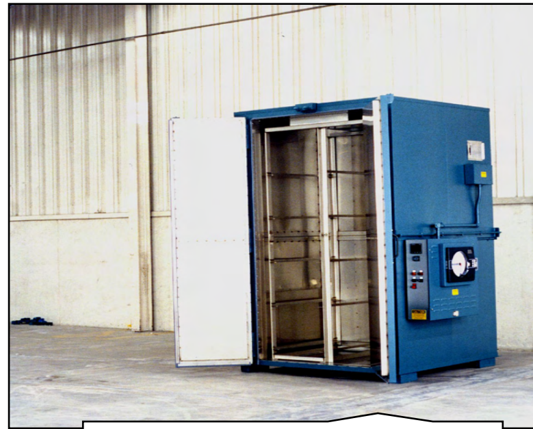
899 Custom Truck Ovens Sectioned
