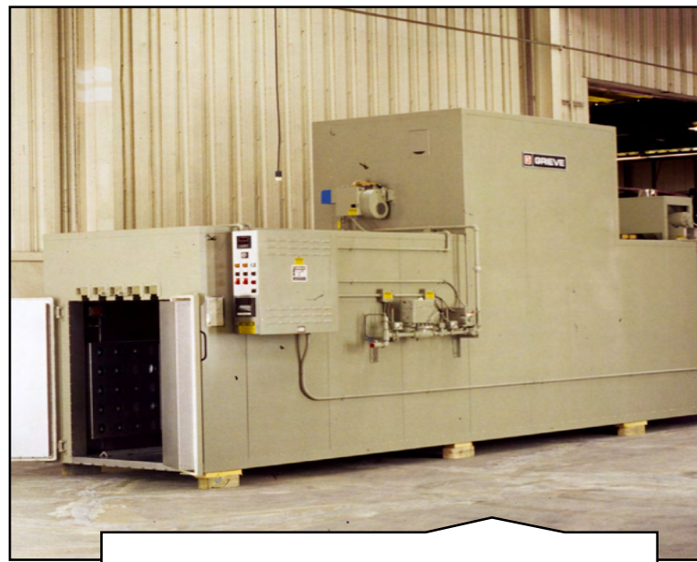
889 Custom Tunnel Walk In Ovens Top Heat Chamber
