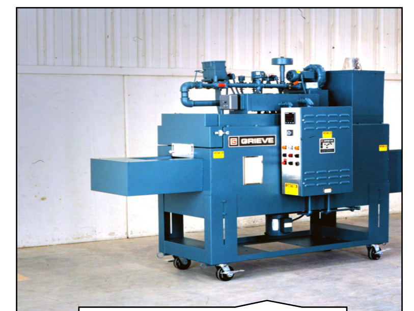
831 Custom Belt Conveyor High Temperature Casters
