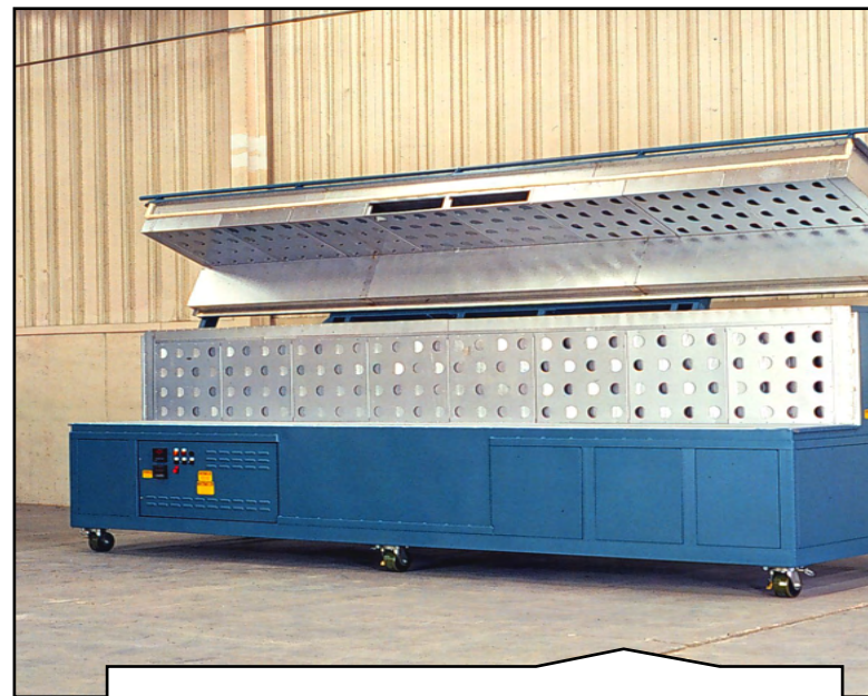
868 Custom Top Loading Casters
