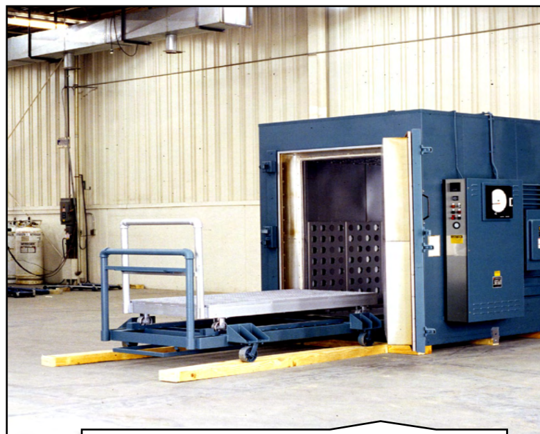
907 Custom Walk In Ovens Inert Atmosphere Truck and Dolly
