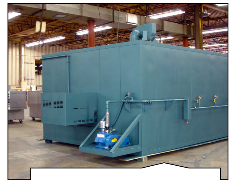
1016 Custom Walk In Ovens Vacuum Manifold
