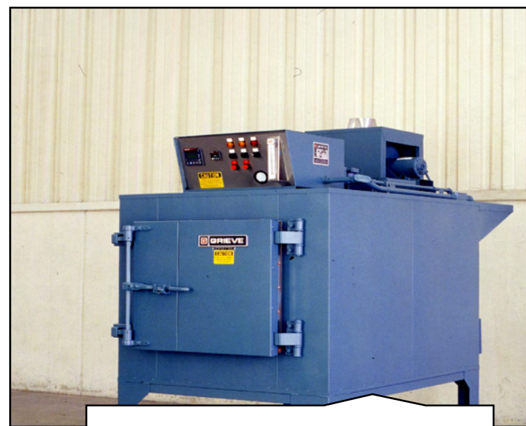
968 Custom Inert Atmosphere
