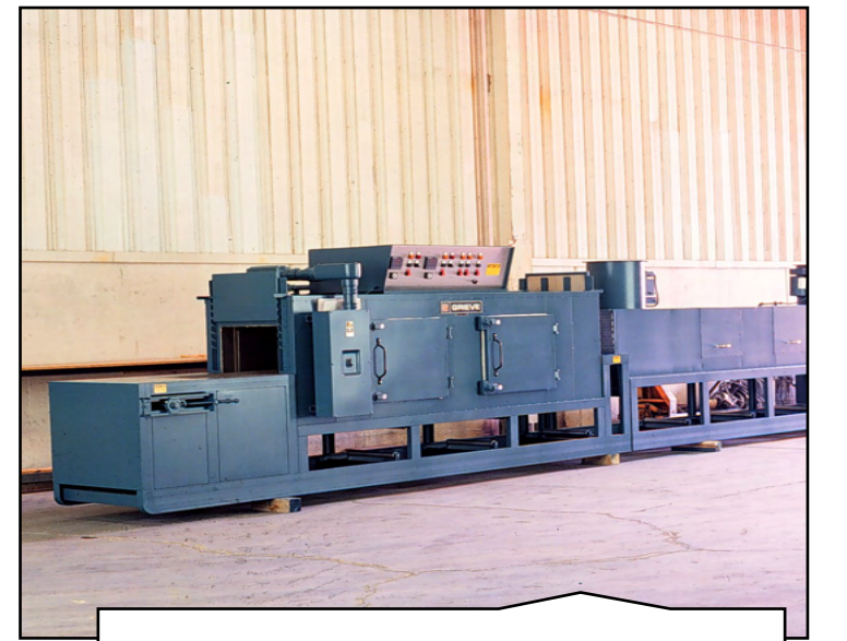
851 Custom Belt Conveyor Zones
