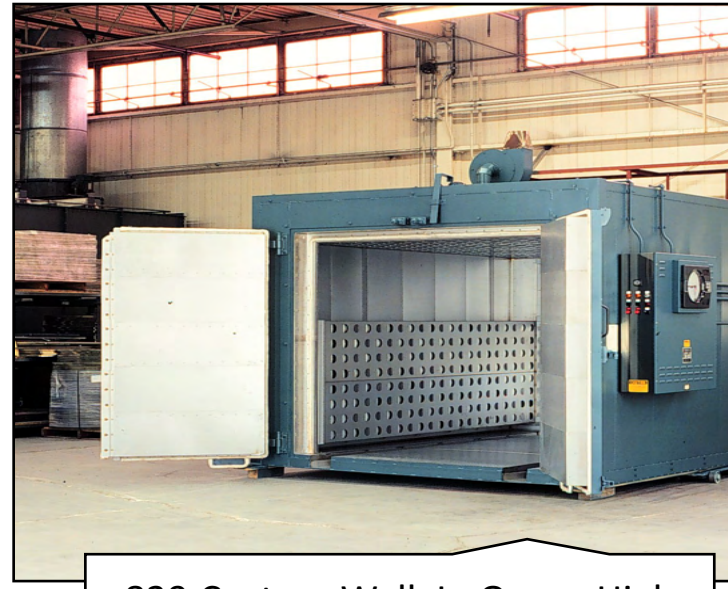
839 Custom Walk In Ovens High Temperature Combination Airflow
